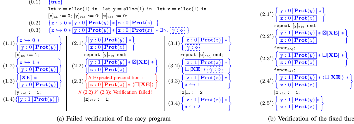
Fig. 11: Verification of Relayed Message Passing
