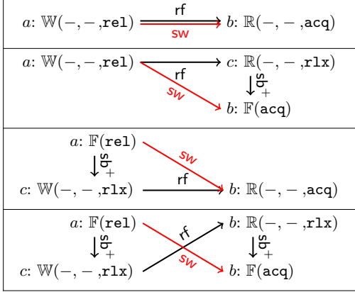
Fig. 5: Four ways to form synchronization
