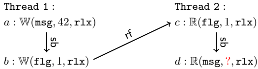
Fig. 7: Failed message passing
