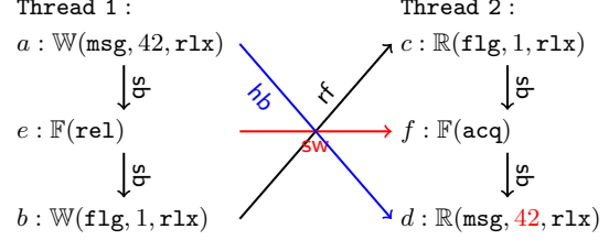
Fig. 8: Message passing using relaxed atomics with fences
